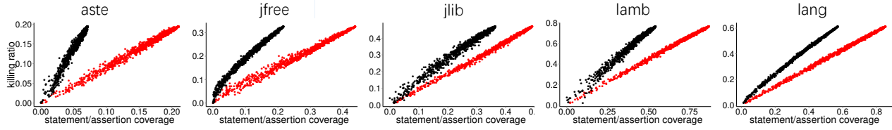
Fig. 2. Results on pseudo test suites. Red/black points are for statement/assertion coverage. In each sub-figure, the horizontal axis represents the corresponding criteria, and the vertical axis represents the fault-revealing ability of test suites (i.e., mutant killing ratio). Each point represents one pseudo test suite. As we can see from the figure, there are very strong correlations between statement/assertion coverage and mutant killing ratio.
